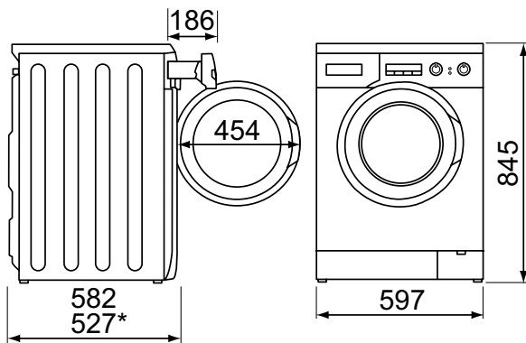
Dimension in millimetres
