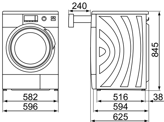
Dimension in millimetres
